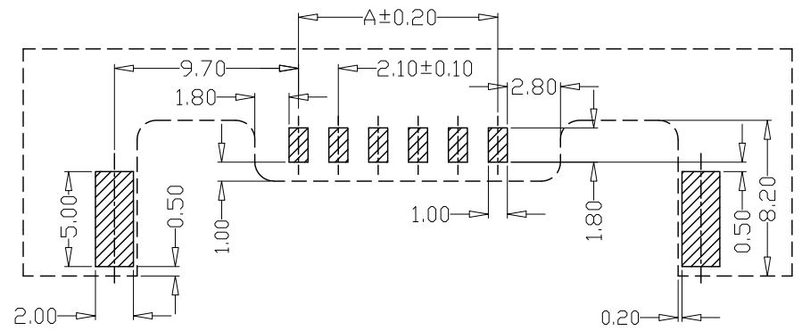
PCB LAYOUT
